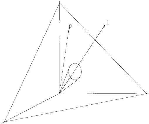
Fig. 1. Schematic view of the situation in which function space \mathcal{F} is three dimensional. The uniform prior over this space, \mathbf{i} , lies along the diagonal. Different algorithms a give different vectors v lying in the cone surrounding the diagonal. A particular problem is represented by its prior \mathbf{p} lying on the simplex. The algorithm that will perform best will be the algorithm in the cone having the largest inner product with \mathbf{p} .
