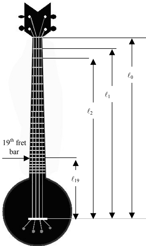
Figure 6: The length of a string from bridge to fret is \ell = \ell_0 . The length, \ell_n , from the bridge to the n^{\text{th}} fret bar is
