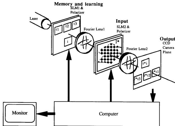
Fig. 4. The optoelectronic ART1 implementation. Input is the pattern i , transformed ( I^* ) and loaded into SLM2. Output is chosen by considering the peak values on the camera plane. The computer controls the SLMs and reads the camera plane.
