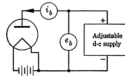
FIG. 2.6. Experimental circuit for measuring diode characteristics.
