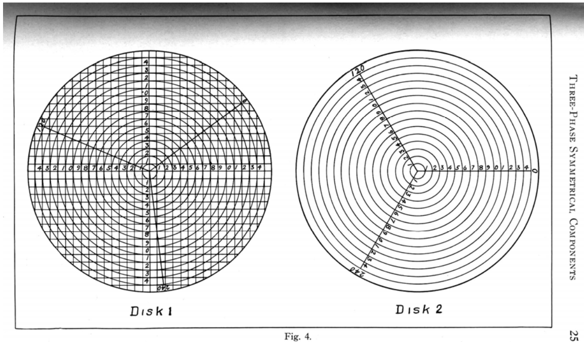
Figure 42. Symmetrical components circular slide rule appearing in Gordon Shuck's Engineering Experiment Station Bulletin No. 84, Equations for Calculating Three Phase Symmetrical Components . Disk 2 was to be transparent and superposed on disk 1. The slide rule was used to quickly find the rectangular coordinates of two phasors in a balanced set when the third is known.
