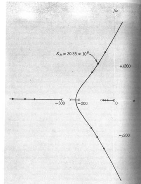
Fig. 7.9. Root locus plot for lead network compensation, P = 300 , Z = 70 .
