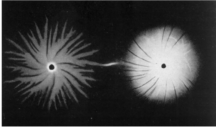
Figure 39. This figure from Magnusson's report Electric Discharges No. 1, Effects of the Magnetic Field on Electric Figures in Air illustrates his main finding. Both positive (left) and negative (right) Lichtenberg figures are created simultaneously on the same photographic plate, placed in a magnetic field. The streamers in each figure spiral in the same direction, indicating that they are made by charges with the same polarity, i.e. electrons. If the positive figure were made by the motion of positive charges, the spiral of the positive figure would be in the opposite direction. The magnetic field is into the page. (Figure from Electric Discharges No. 1, Effects of the Magnetic Field on Electric Figures in Air )
