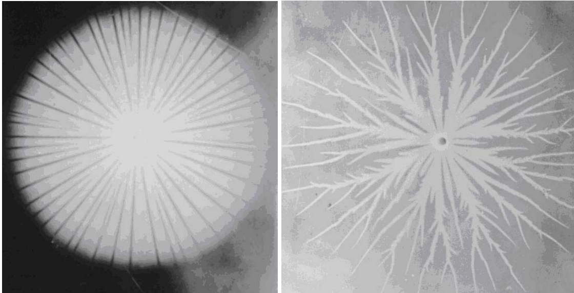
Figure 38. Lichtenberg figures created by discharging the negative terminal (left) and positive terminal (right) of a capacitor through a spark gap. The difference in the appearance of the figures gave rise to the theory that the negative terminal emitted negative charges (electrons) and the positive terminal emitted positive charges (ions). Professor Magnusson demonstrated that negative charges were emitted in both cases.
