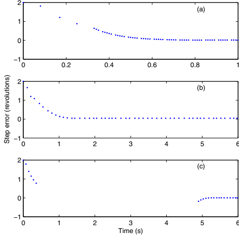
Fig. 1. Step responses for the three cases discussed in the text. Note that the time axis in case (a) has been magnified in order to see the individual points in the time scale.
